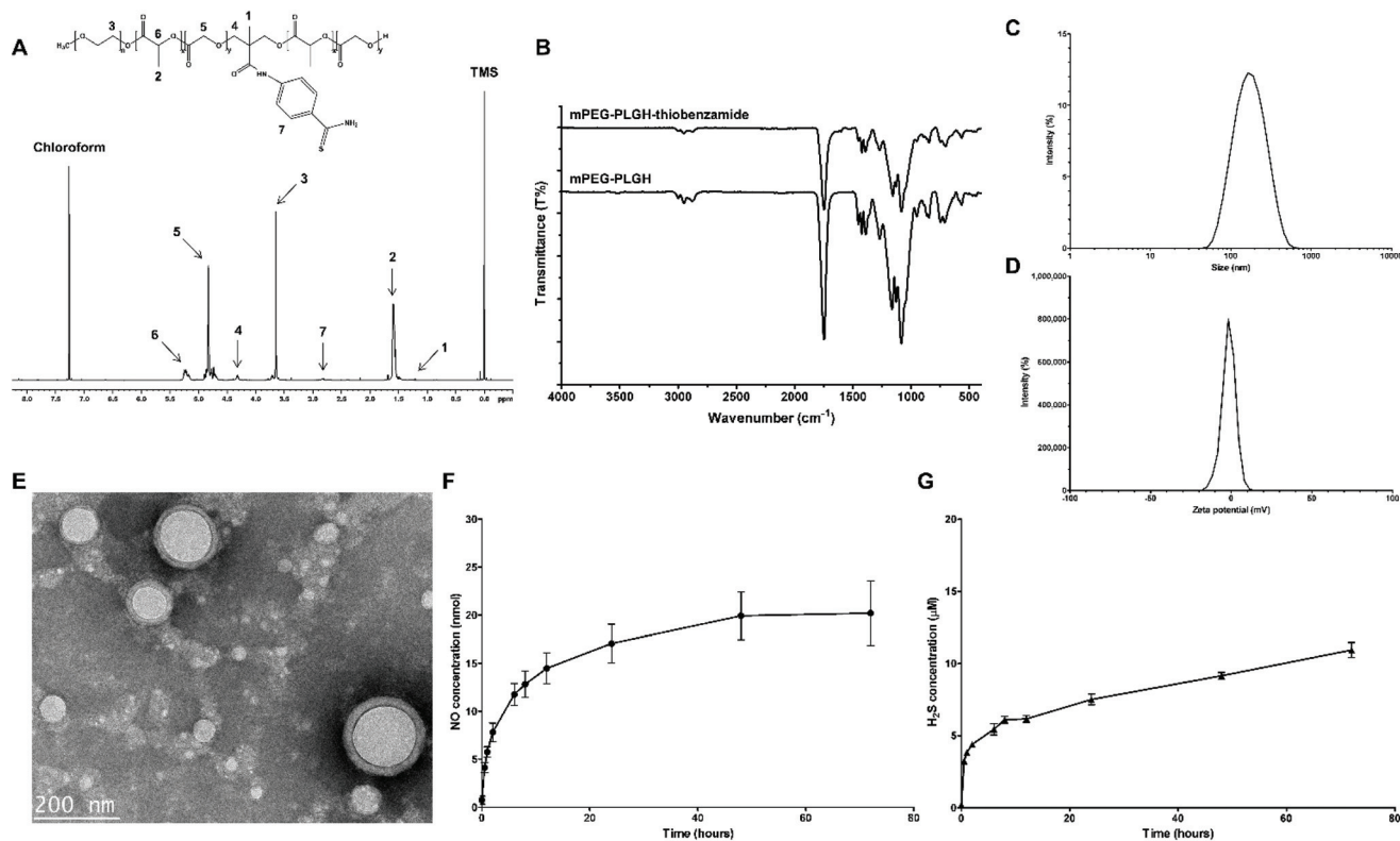
Fig. 2 Characterization of the PTA copolymers and PTA-NO-NPs. (A) ^1\text{H} NMR spectrum of the PTA copolymers with \text{d} -chloroform as a solvent. (B) FT-IR spectra of the mPEG-PLGH and PTA copolymers. (C) Size distribution and (D) zeta potential confirmed by DLS. The data are displayed as the mean \pm SEM ( n = 4 ). (E) Morphological analysis was determined by TEM. The scale bar is 200 nm. (F) Nitric oxide release measurement by Griess assay and (G) Hydrogen sulfide release measurement by the methylene blue method were carried out in vitro . PTA-NO-NPs at 1 \text{ mg ml}^{-1} were tested under physiological conditions. The data are displayed as the mean \pm SEM ( n = 3 ).
