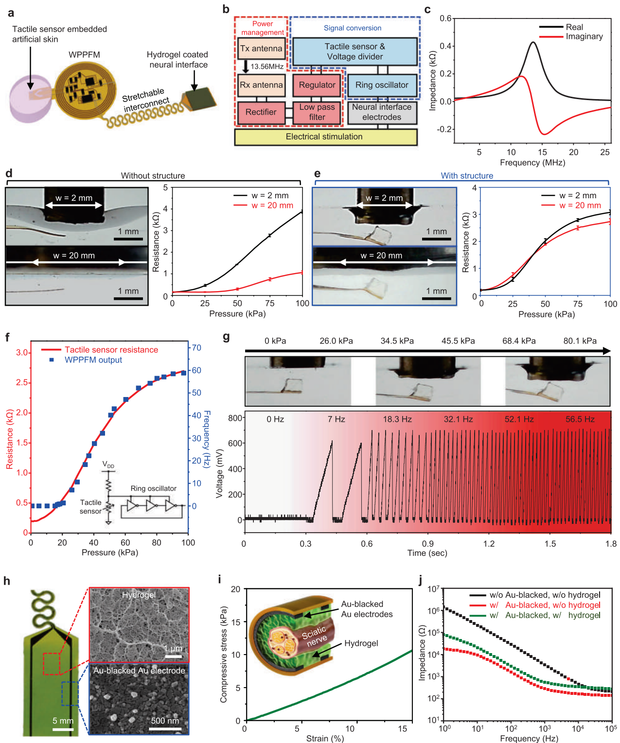
Fig. 2 | Characteristics of the WPPFM and neural interface electrodes.
