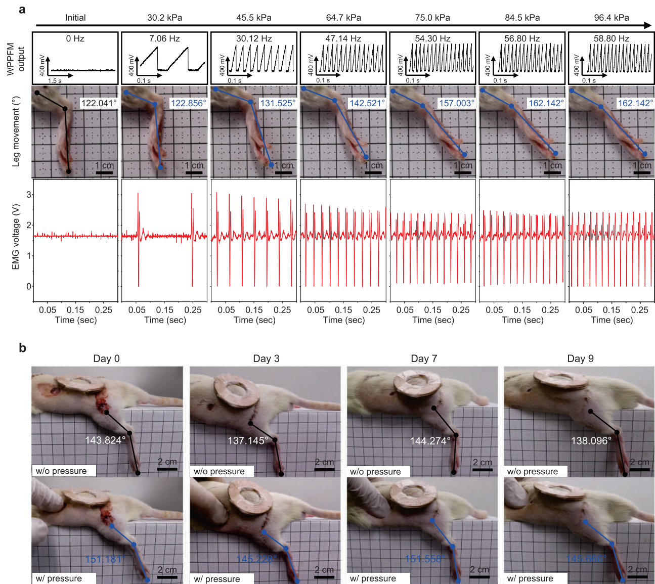
Fig. 5 | In vivo demonstration of implanted WTSA and precise analysis of leg movements according to the externally applied pressure. a Quantitative analysis of leg movement angle (blue line) and electromyogram signal (red) monitoring while different pressure is applied (Initial, 30.2, 45.5, 64.7, 75.0, 84.5, and 96.4 kPa). Inset black box represents the output signal from WPPFM, and the inset
